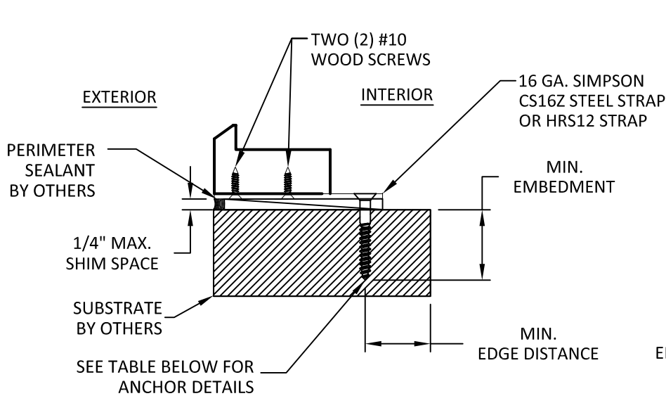
B 11 VERTICAL SECTION STRAP - SILL SHOWN, HEAD/JAMB SIM.
