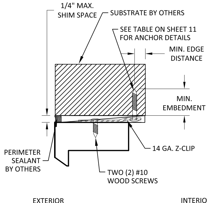
C 10 VERTICAL SECTION INTERIOR Z-CLIP - HEAD SHOWN, JAMB/SILL SIMILAR
